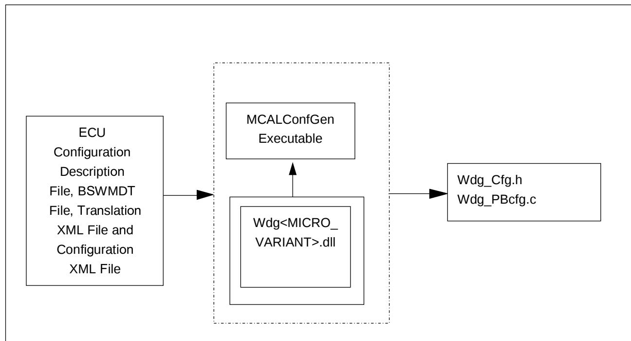
Figure 14-1 Overview of WDG Driver Generation Tool
