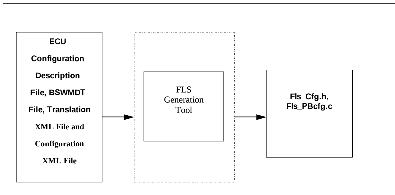
Figure 8.1 Overview of FLS Driver Generation Tool
