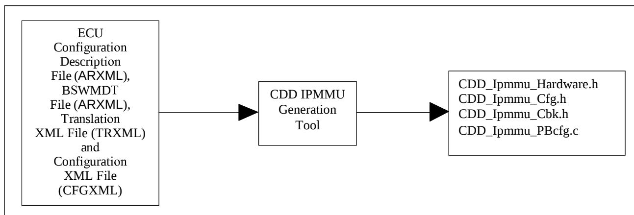
Figure 16-1 Overview of IPMMU Complex Device Driver Generation Tool
