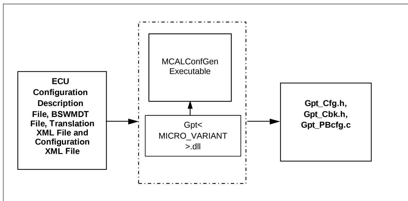
Figure 9.1 Overview of GPT Driver Generation Tool
