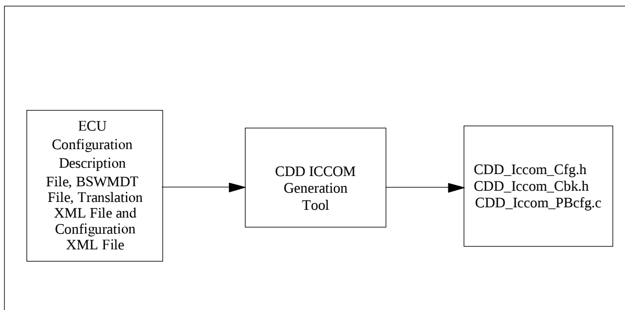
Figure 10.1 Overview of ICCOM Complex Device Driver Generation Tool
