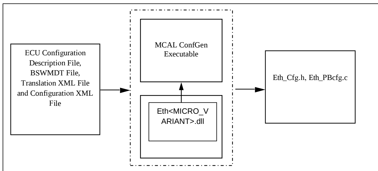
Figure 7.1 Overview of ETH Driver Generation Tool
