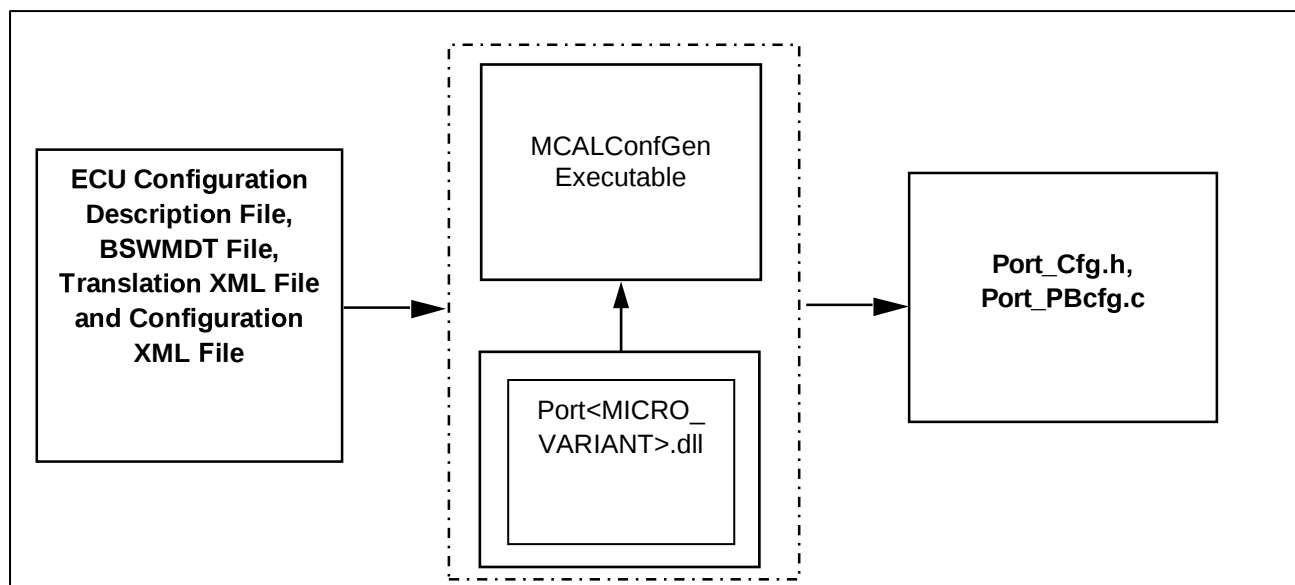
Figure 6.1 Overview of PORT Driver Generation Tool
